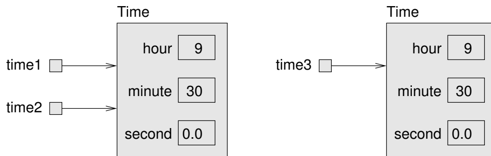
Figure 12.2: Memory diagram of three Time variables.
