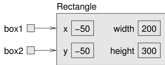
Figure 11.5: Memory diagram showing the effect of invoking grow .
